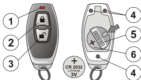
Figure: 1–LED indicator; 2–setting (ON) button; 3–unsetting (OFF) button; 4–bottom cover screws; 5–production code; 6–CR2032 battery (remove the battery by pressing it in the direction of the arrow).
